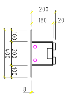
TYPSEKTION 200:200/400x8/60x20
